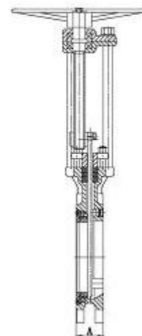
Inside screw nonrising stem type
