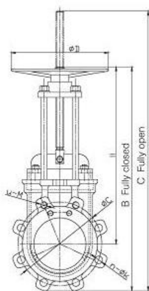
Outside screw rising stem type
